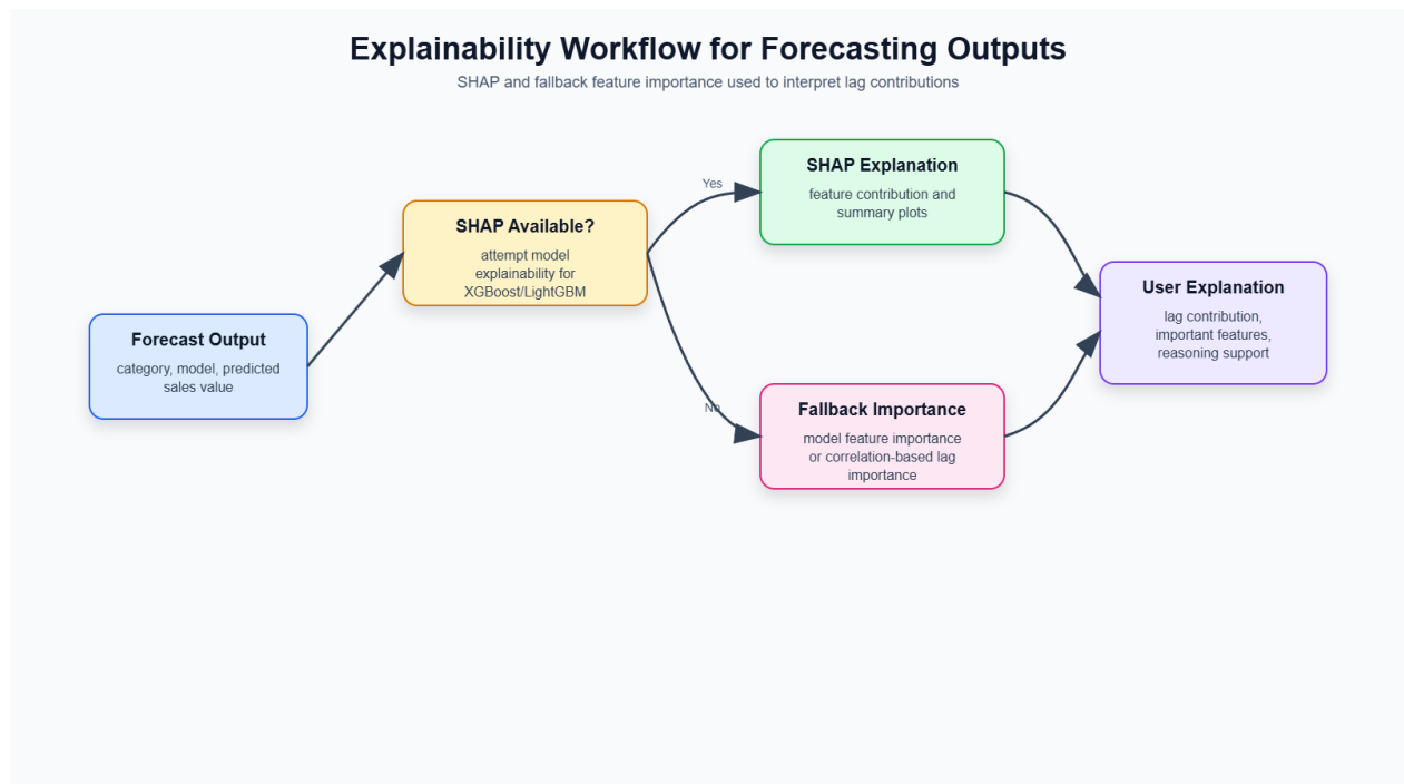
Figure 3:8: Explainability Workflow for Forecasting Outputs
